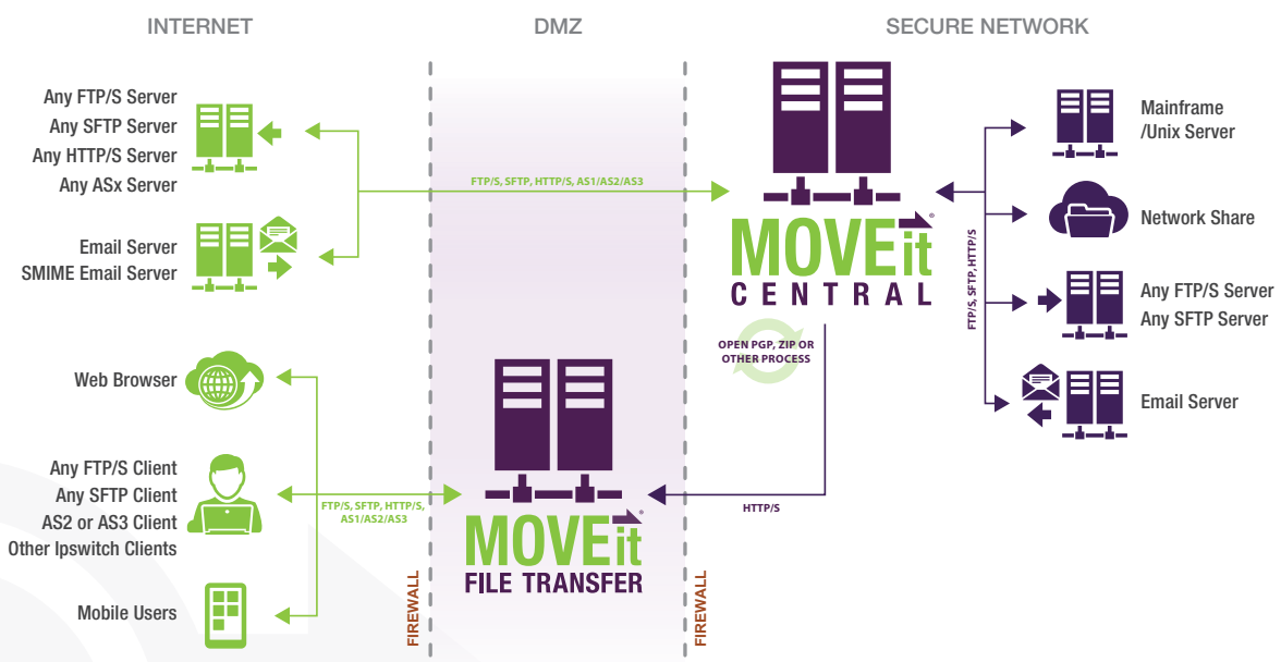
MOVEit Central Architecture
